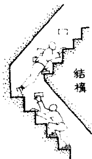
SECTION THRU STAIRWAY PAGODA, KUANG-SHENG SSU, CHAO-CH'ENG, SHANSI
