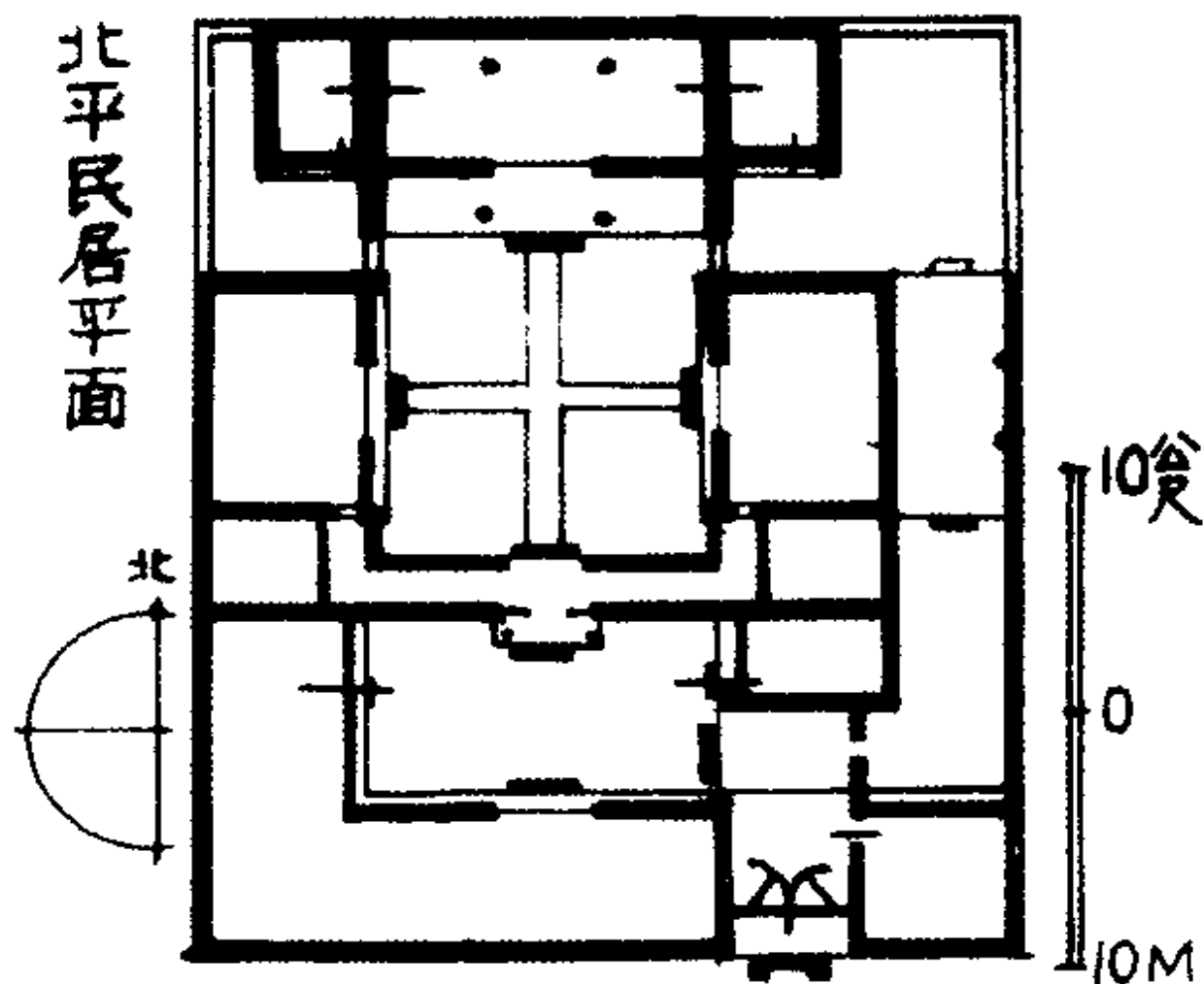
PLAN OF A RESIDENCE, PEIPING.
