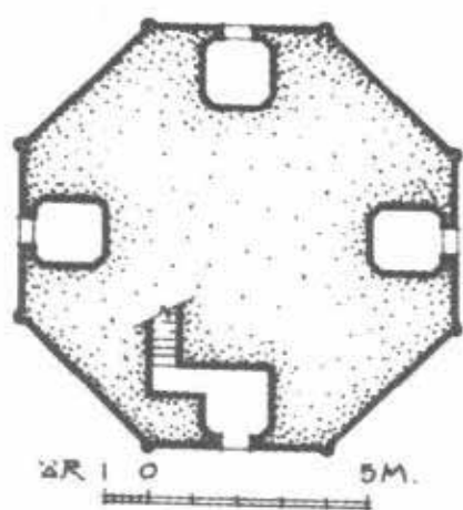
河南開封市祐國寺铁塔平面圖 PLAN OF "IRON PAGODA" YIU-KUO SSU, KAI-FENG, HONAN
